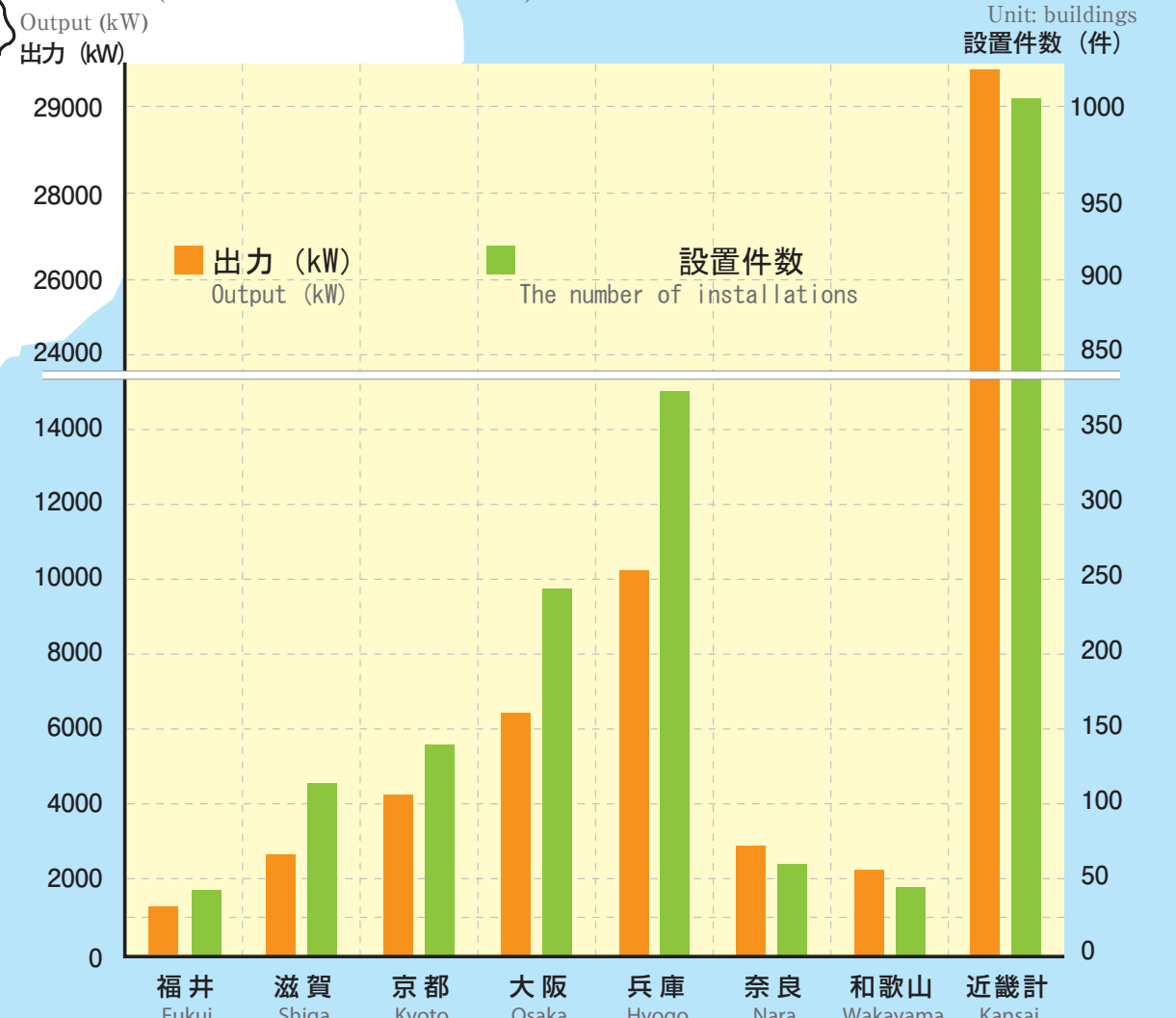
●近畿地域公共・産業用太陽光発電システム導入事例 (平成19年度累積) Introduction of PV generation systems for public facilities and industrial buildings in Kansai area (Cumulative numbers until FY 2007)
